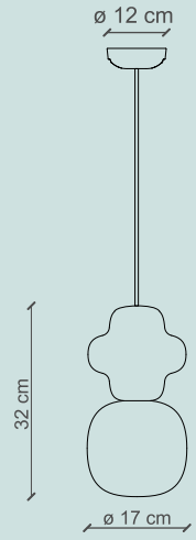
art. C2681 peso netto / net weight 2,12 1 x MAX 28W E14
